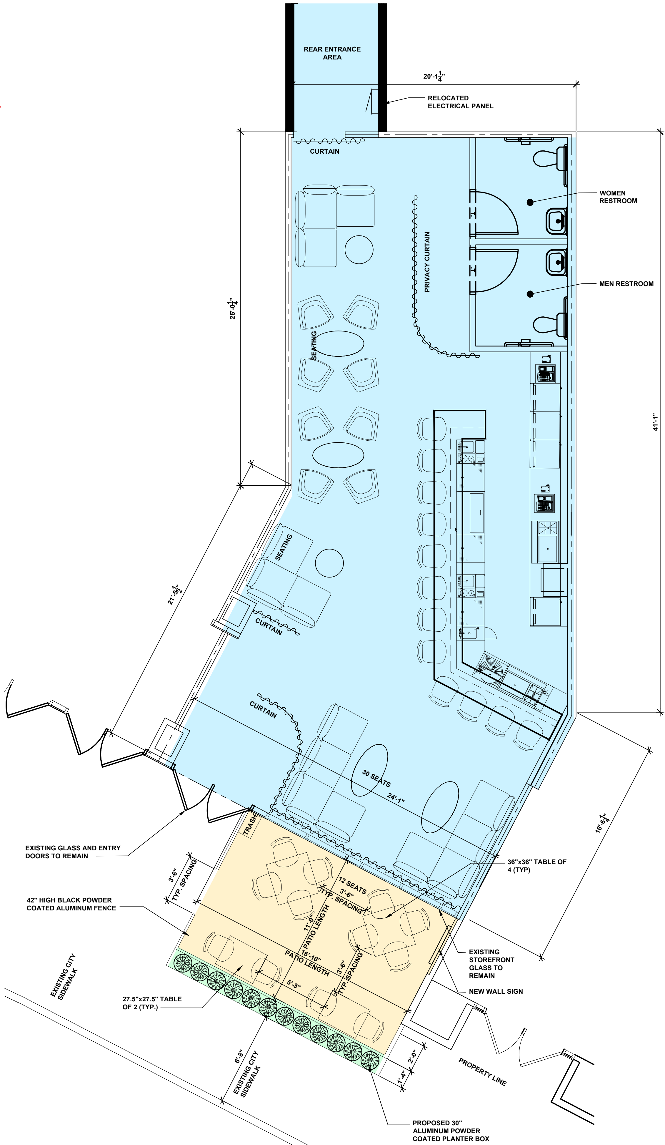
101.01 A.101 NORTH FLOOR PLAN SCALE: 1/4"=1'-0"
